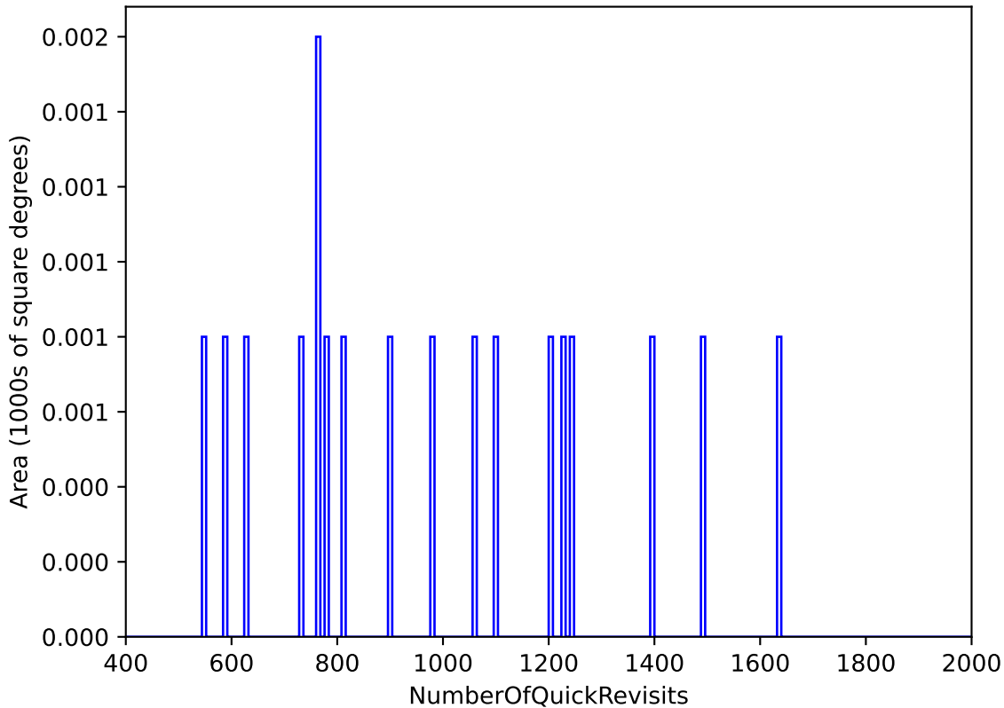
too_elab_heavy_r32_d2_ugrizy_v3.4_10yrs WFD: NumberOfQuickRevisits
