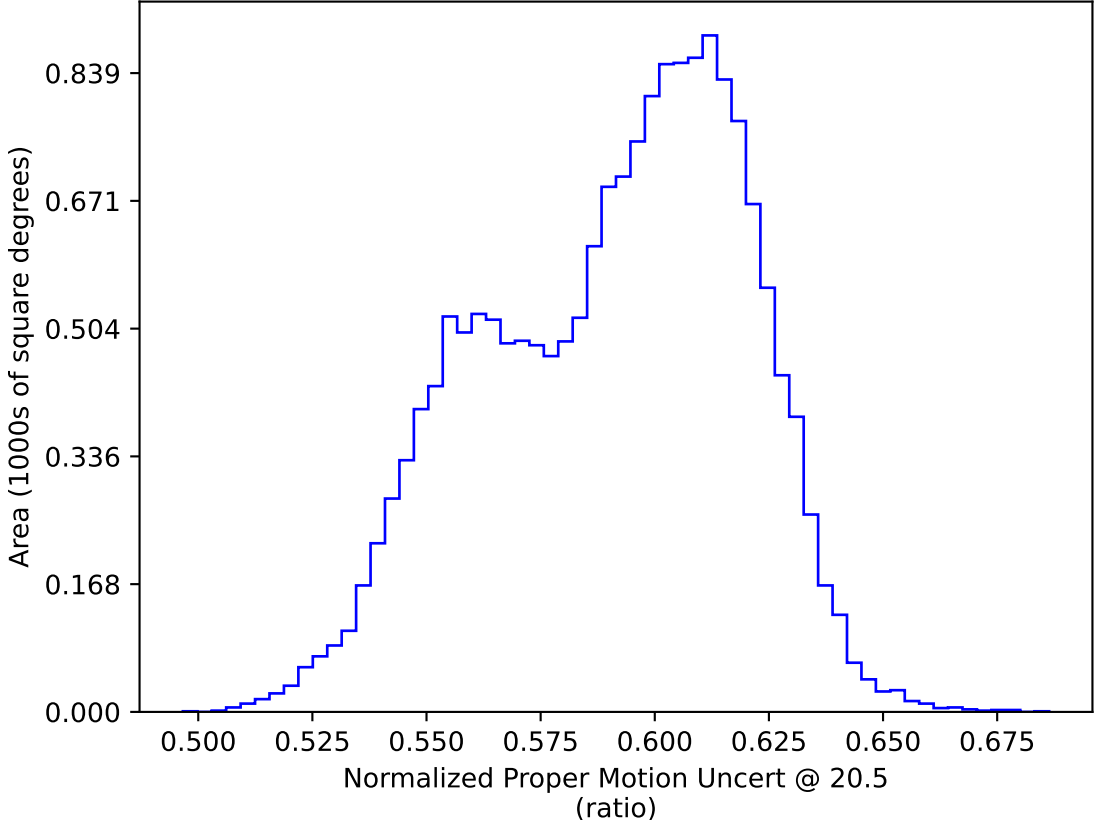
too_elab_heavy_r32_d2_ugrizy_v3.4_10yrs WFD: Normalized Proper Motion Uncert @ 20.5
