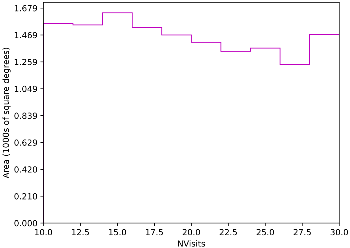
too_elab_heavy_r32_d2_ugrizy_v3.4_10yrs Yr 3-4 z band: NVisits
