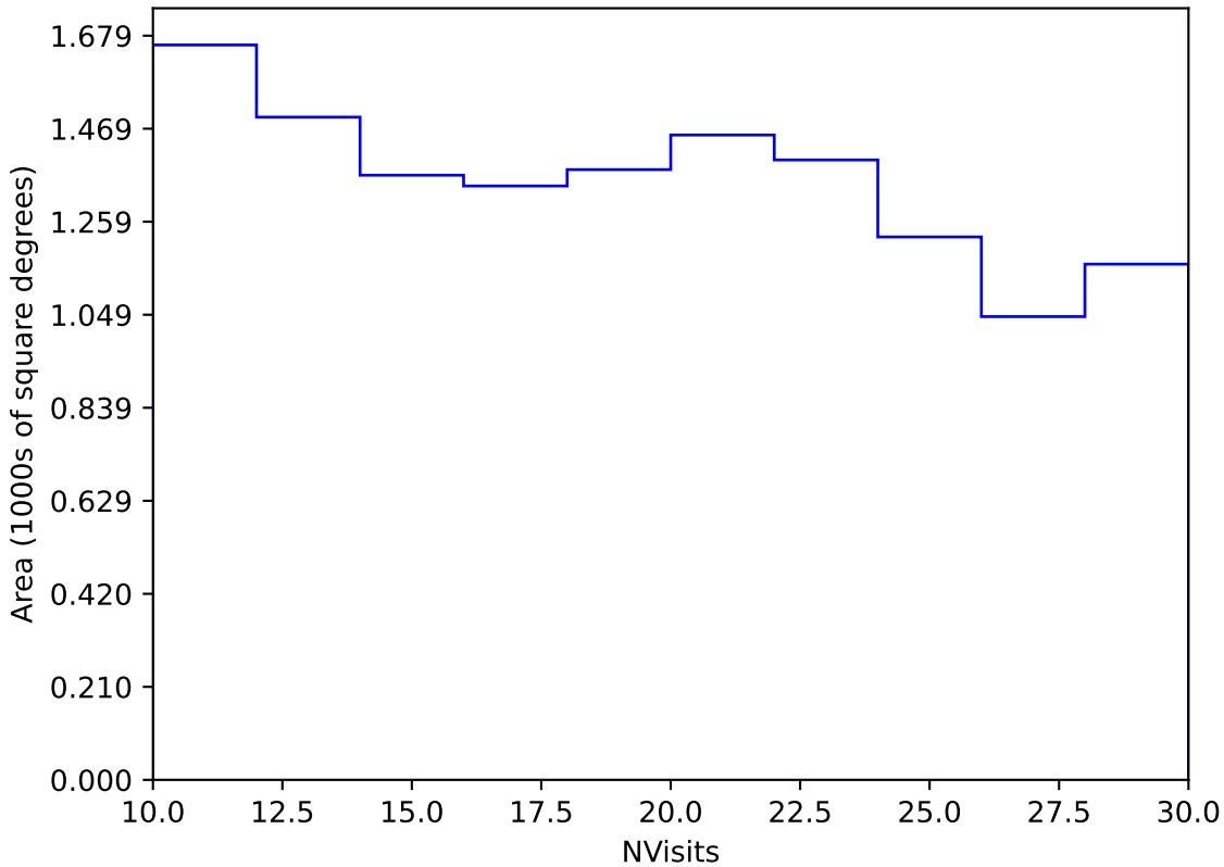
too_elab_heavy_r32_d2_ugrizy_v3.4_10yrs Yr 3-4 y band: NVisits
