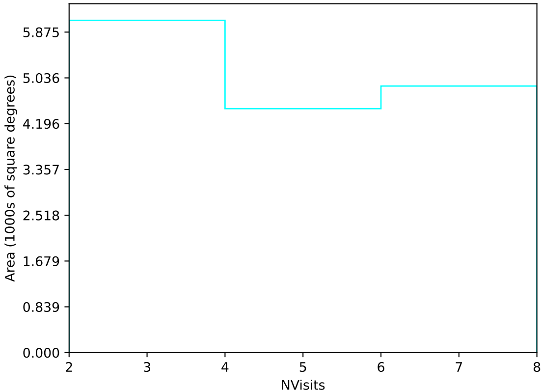
too_elab_heavy_r32_d2_ugrizy_v3.4_10yrs Yr 3-4 u band: NVisits
