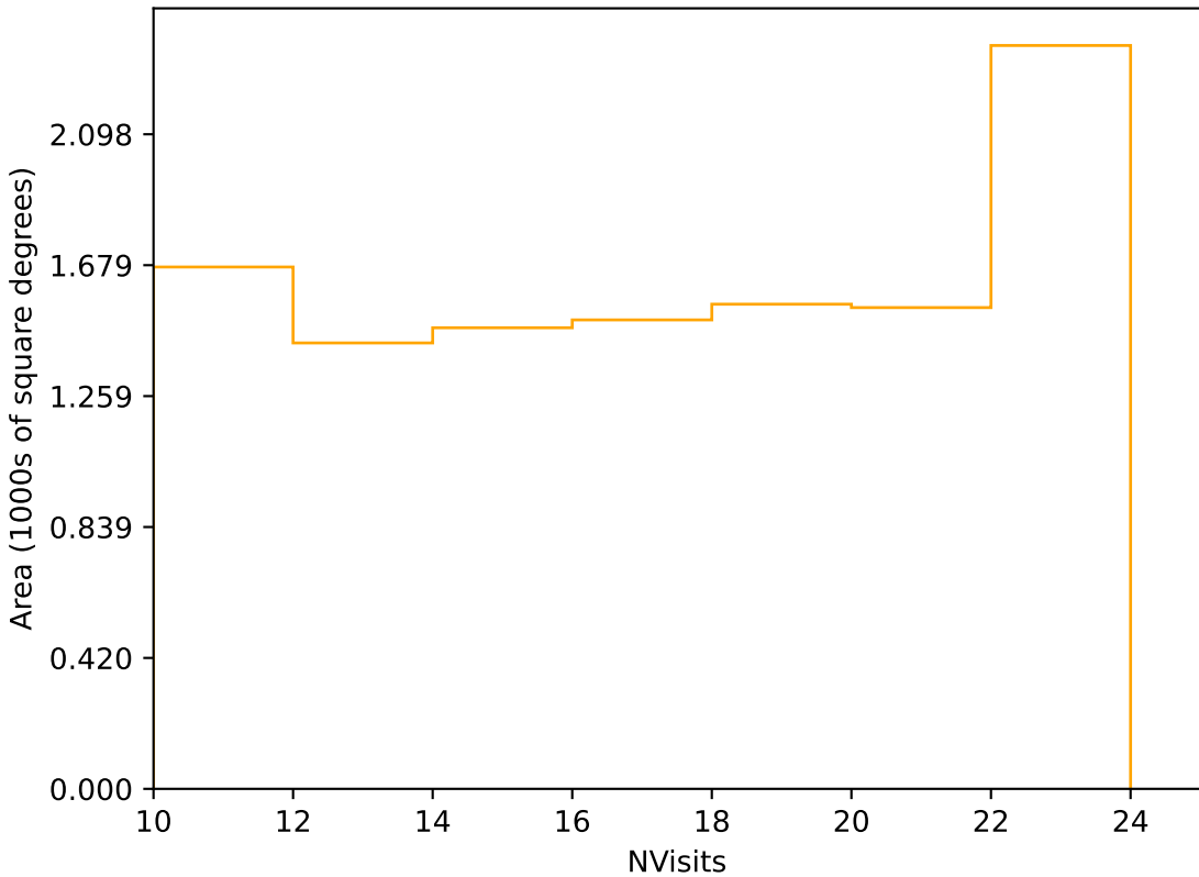
too_elab_heavy_r32_d2_ugrizy_v3.4_10yrs Yr 3-4 r band: NVisits
