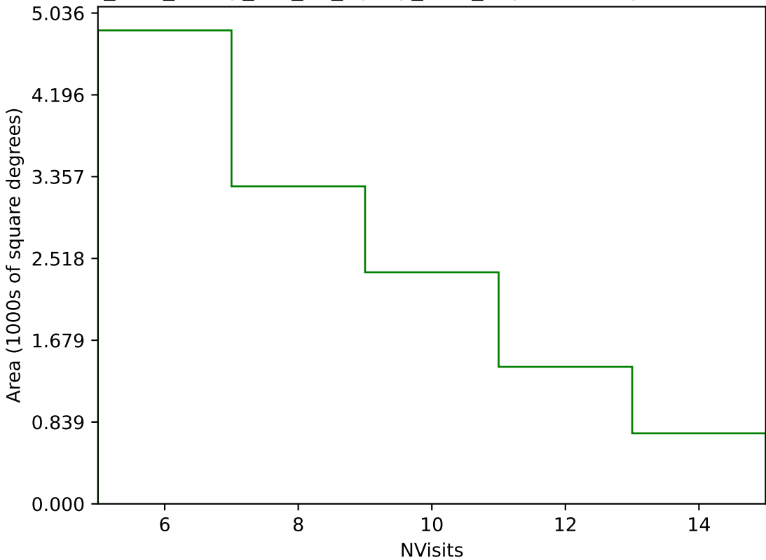
too_elab_heavy_r32_d2_ugrizy_v3.4_10yrs Yr 3-4 g band: NVisits
