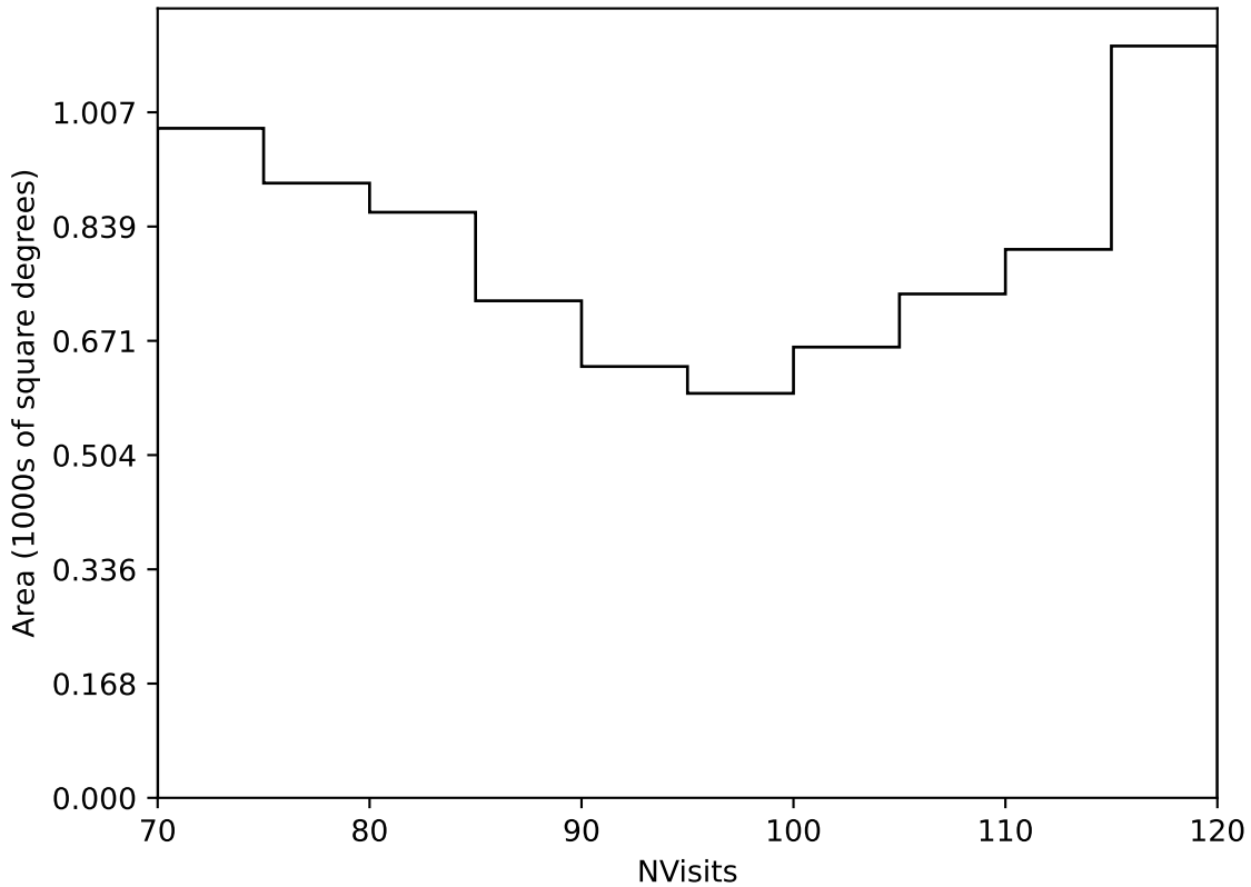
too_elab_heavy_r32_d2_ugrizy_v3.4_10yrs Yr 3-4 all bands: NVisits
