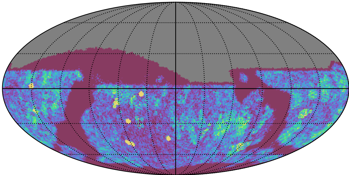
too_elab_heavy_r32_d2_ugrizy_v3.4_10yrs Yr 1 z band: NVisits
