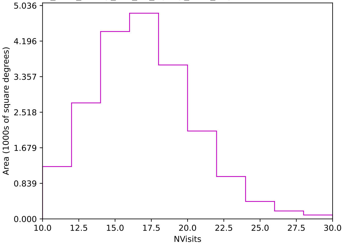
too_elab_heavy_r32_d2_ugrizy_v3.4_10yrs Yr 1 z band: NVisits
