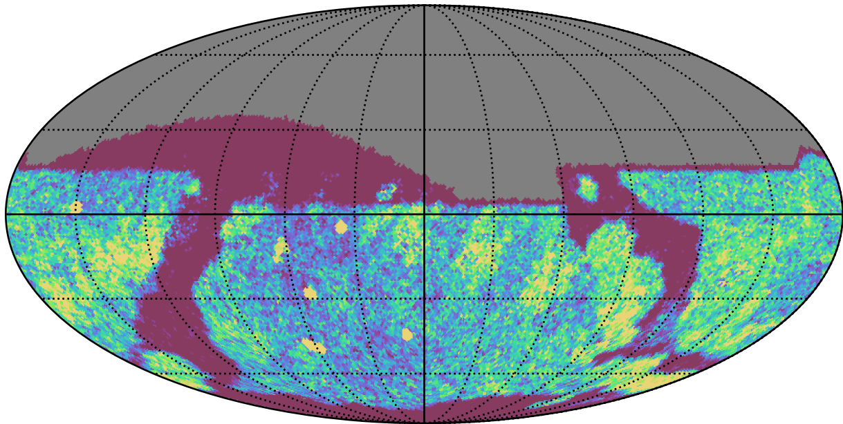
too_elab_heavy_r32_d2_ugrizy_v3.4_10yrs Yr 1 r band: NVisits
