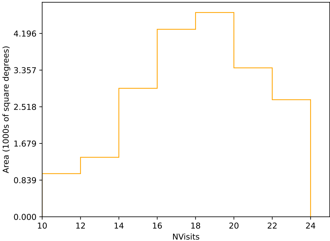
too_elab_heavy_r32_d2_ugrizy_v3.4_10yrs Yr 1 r band: NVisits
