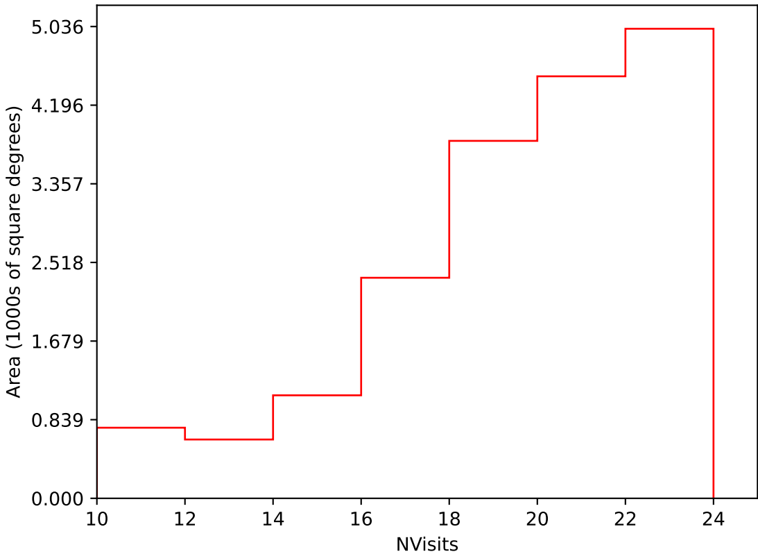
too_elab_heavy_r32_d2_ugrizy_v3.4_10yrs Yr 1 i band: NVisits
