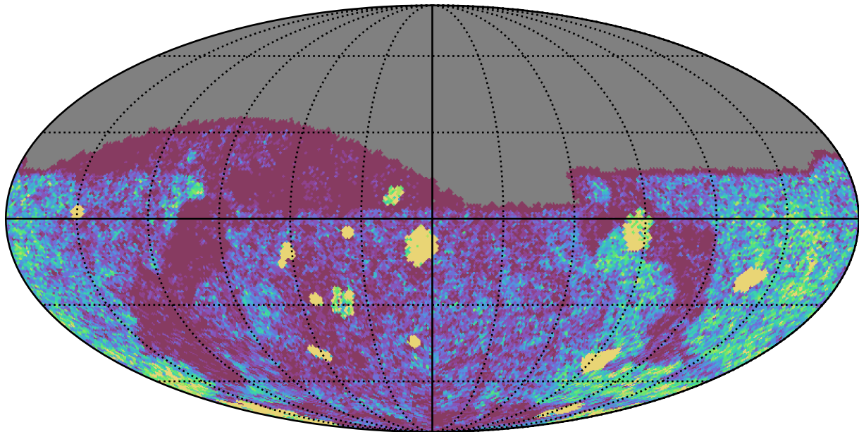
too_elab_heavy_r32_d2_ugrizy_v3.4_10yrs Yr 1 g band: NVisits
