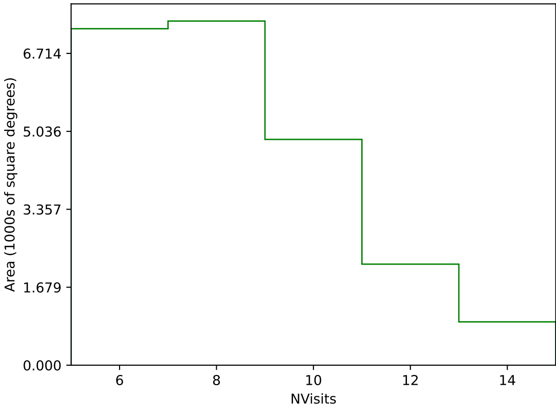
too_elab_heavy_r32_d2_ugrizy_v3.4_10yrs Yr 1 g band: NVisits
