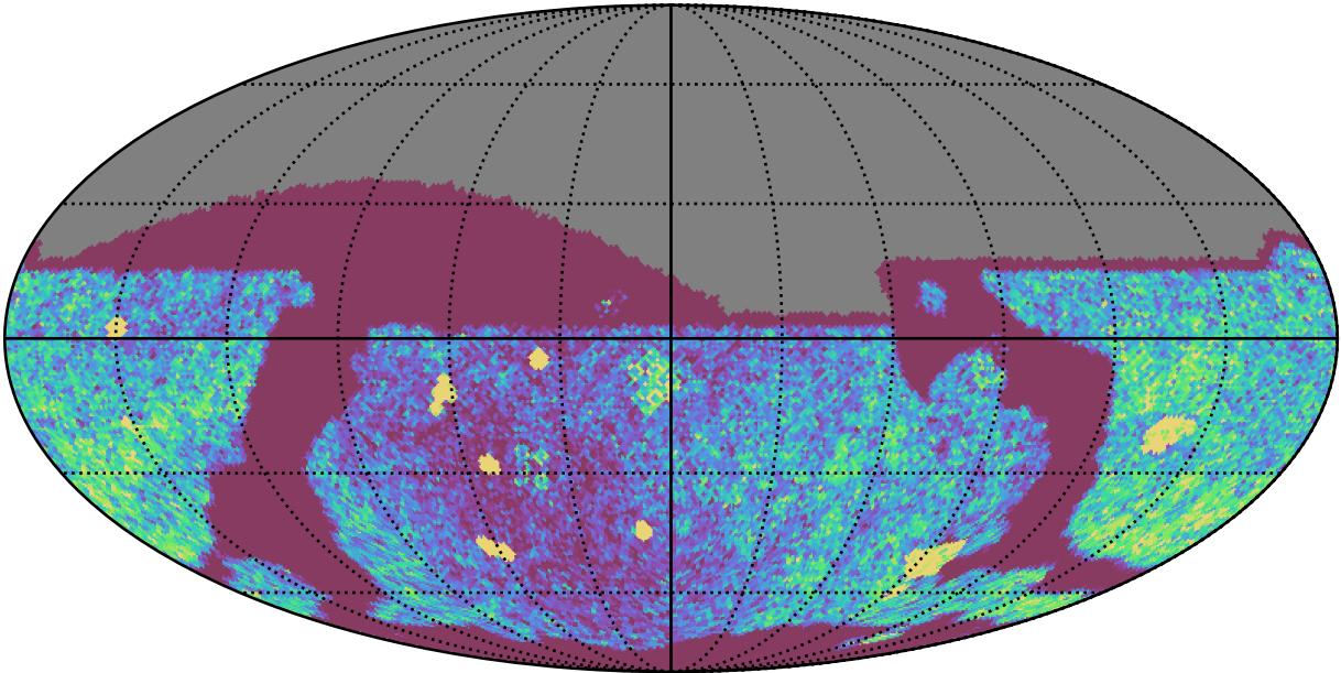
too_elab_heavy_r32_d2_ugrizy_v3.4_10yrs Yr 1 all bands: NVisits
