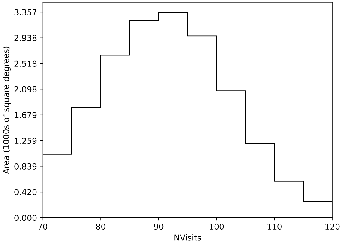
too_elab_heavy_r32_d2_ugrizy_v3.4_10yrs Yr 1 all bands: NVisits
