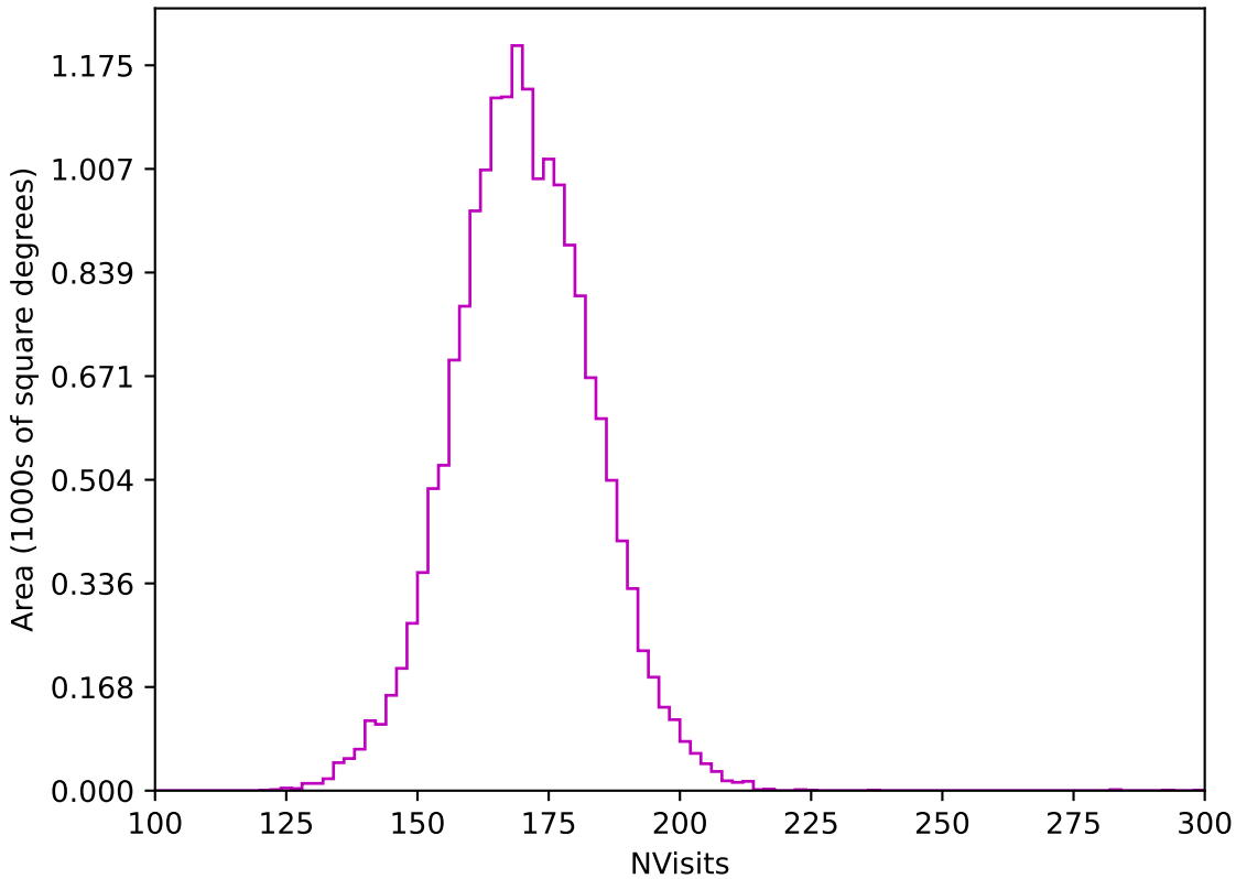
too_elab_heavy_r32_d2_ugrizy_v3.4_10yrs WFD z band: NVisits
