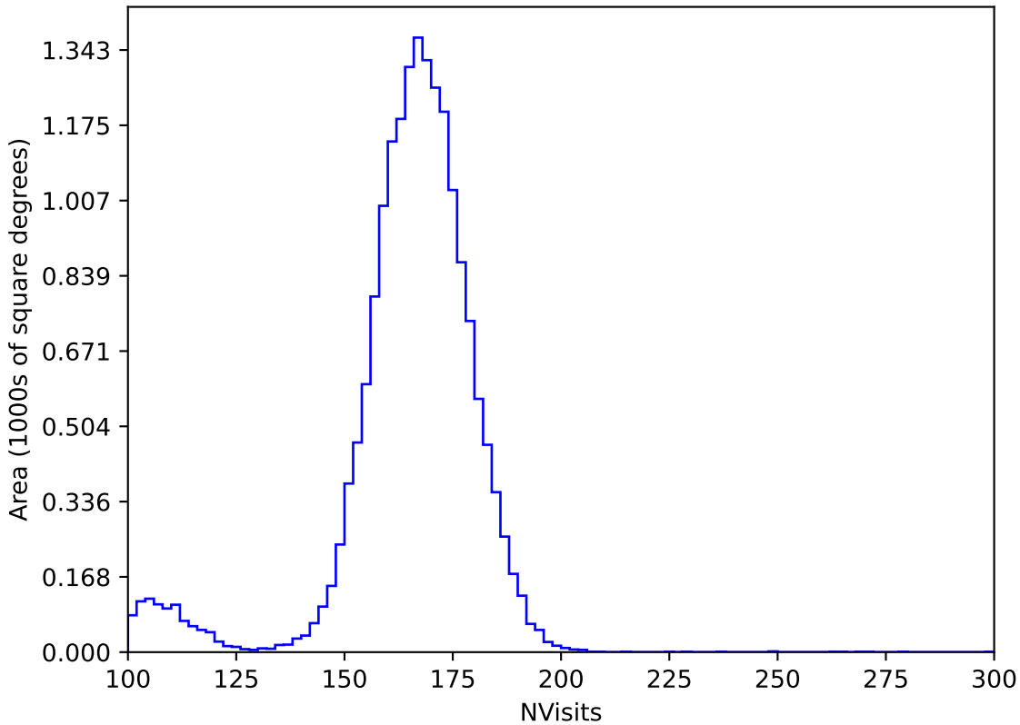
too_elab_heavy_r32_d2_ugrizy_v3.4_10yrs WFD y band: NVisits
