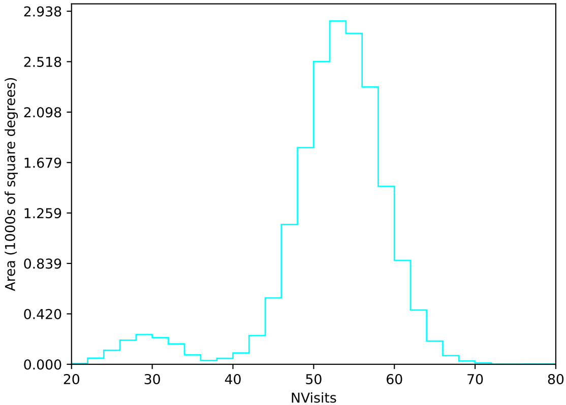
too_elab_heavy_r32_d2_ugrizy_v3.4_10yrs WFD u band: NVisits
