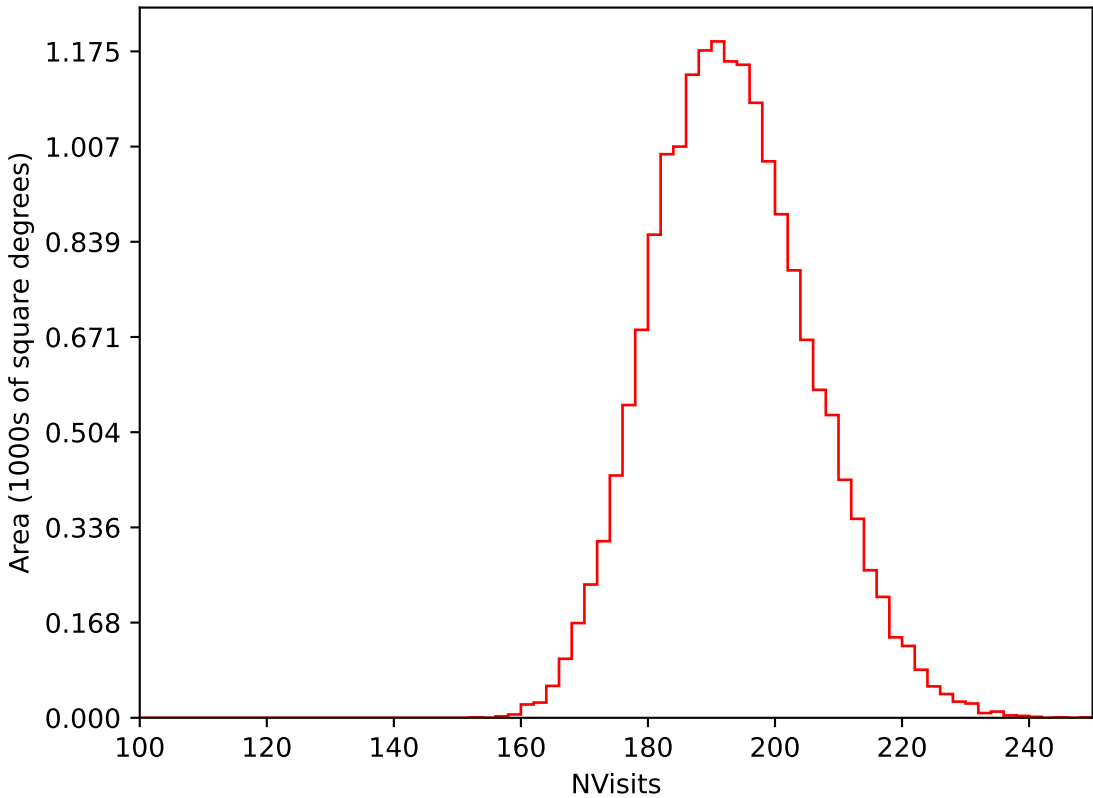
too_elab_heavy_r32_d2_ugrizy_v3.4_10yrs WFD i band: NVisits
