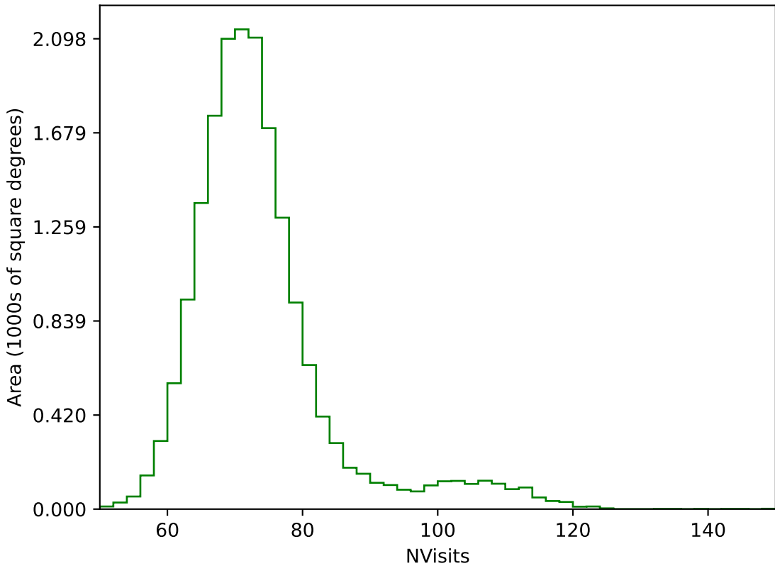
too_elab_heavy_r32_d2_ugrizy_v3.4_10yrs WFD g band: NVisits
