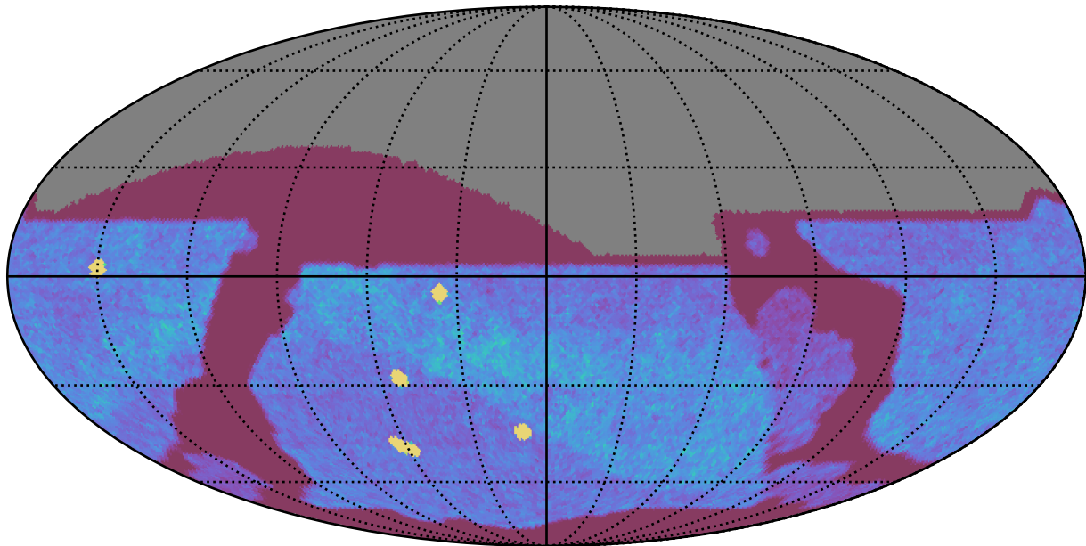
too_elab_heavy_r32_d2_ugrizy_v3.4_10yrs All sky z band: NVisits
