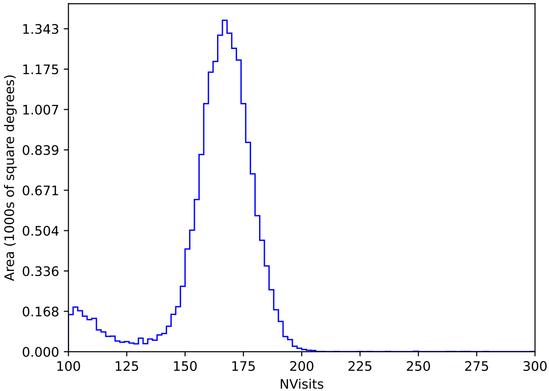
too_elab_heavy_r32_d2_ugrizy_v3.4_10yrs All sky y band: NVisits
