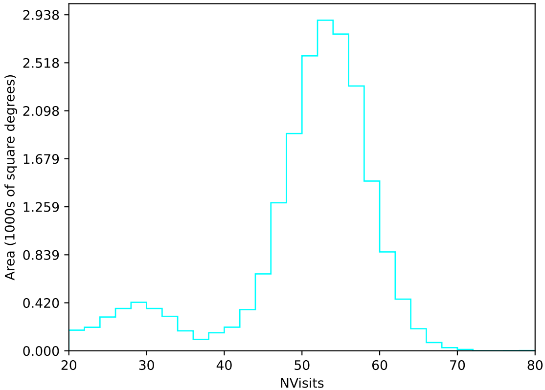
too_elab_heavy_r32_d2_ugrizy_v3.4_10yrs All sky u band: NVisits
