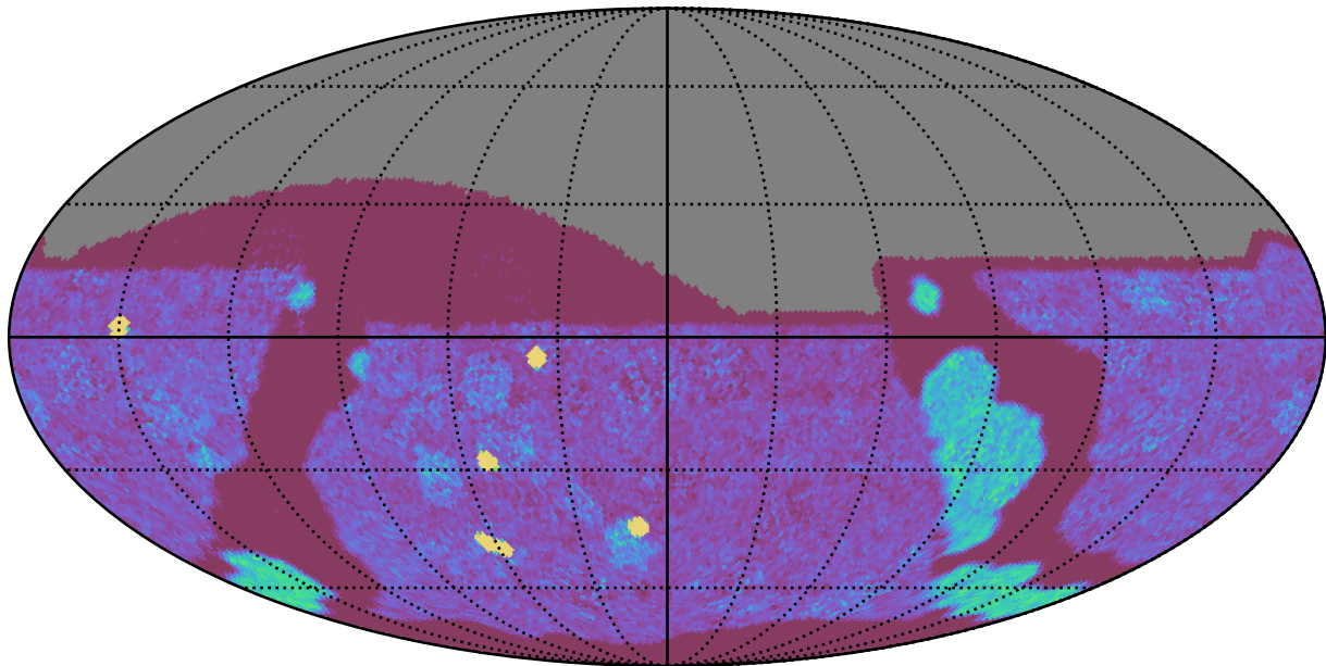
too_elab_heavy_r32_d2_ugrizy_v3.4_10yrs All sky g band: NVisits
