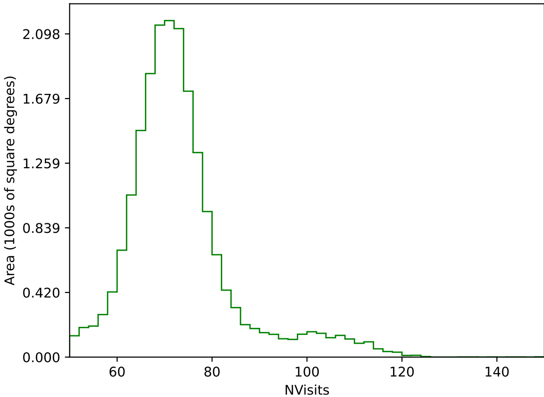
too_elab_heavy_r32_d2_ugrizy_v3.4_10yrs All sky g band: NVisits
