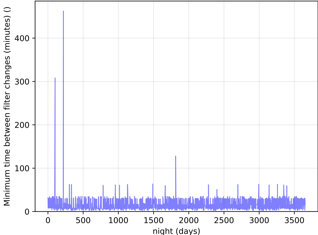
too_elab_heavy_r32_d2_ugrizy_v3.4_10yrs Per Night: Minimum time between filter changes (minutes)
