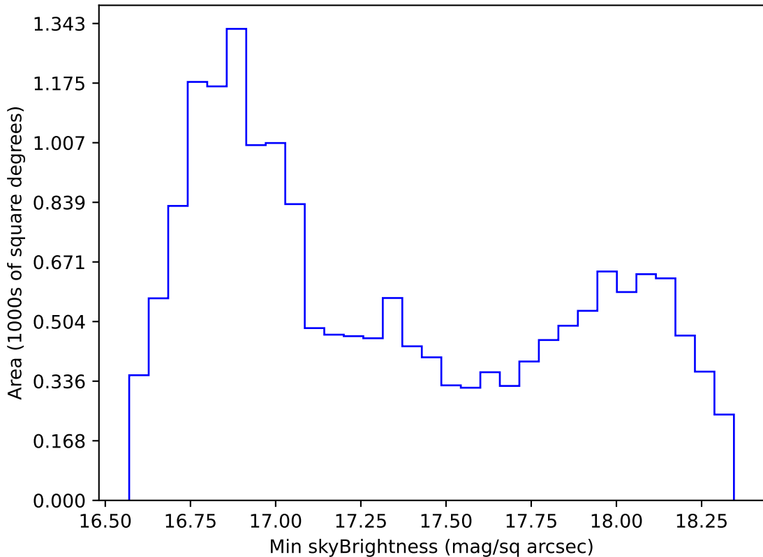
too_elab_heavy_r32_d2_ugrizy_v3.4_10yrs WFD z band: Min skyBrightness
