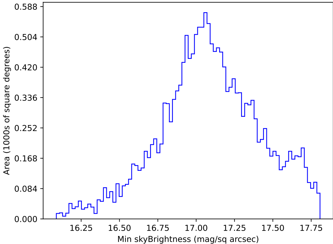
too_elab_heavy_r32_d2_ugrizy_v3.4_10yrs WFD y band: Min skyBrightness
