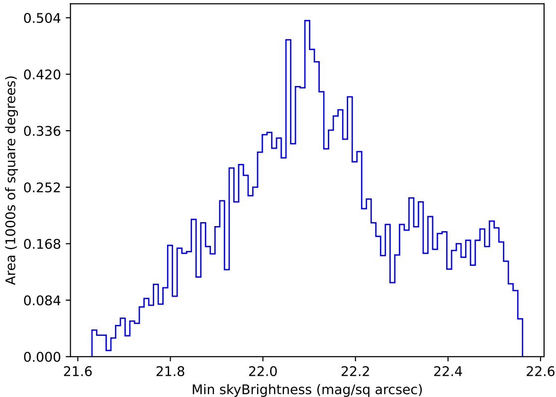
too_elab_heavy_r32_d2_ugrizy_v3.4_10yrs WFD u band: Min skyBrightness
