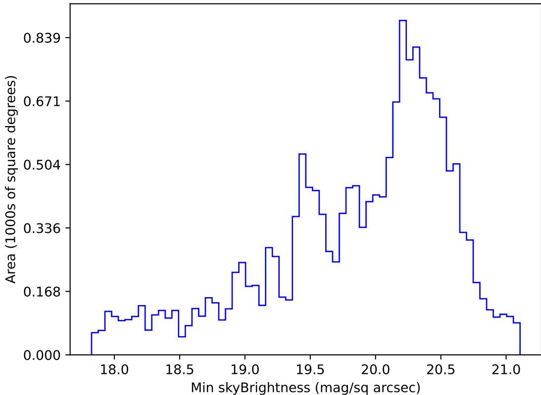
too_elab_heavy_r32_d2_ugrizy_v3.4_10yrs WFD g band: Min skyBrightness
