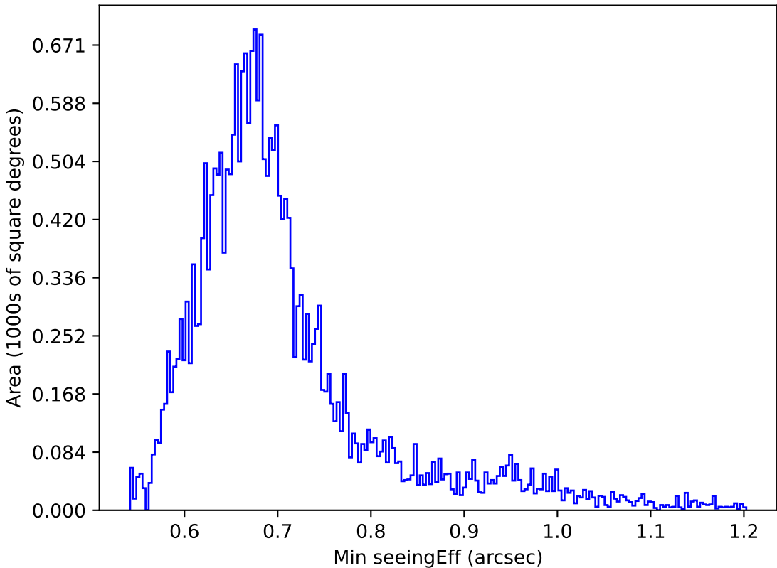
too_elab_heavy_r32_d2_ugrizy_v3.4_10yrs Yr 1 i band: Min seeingEff
