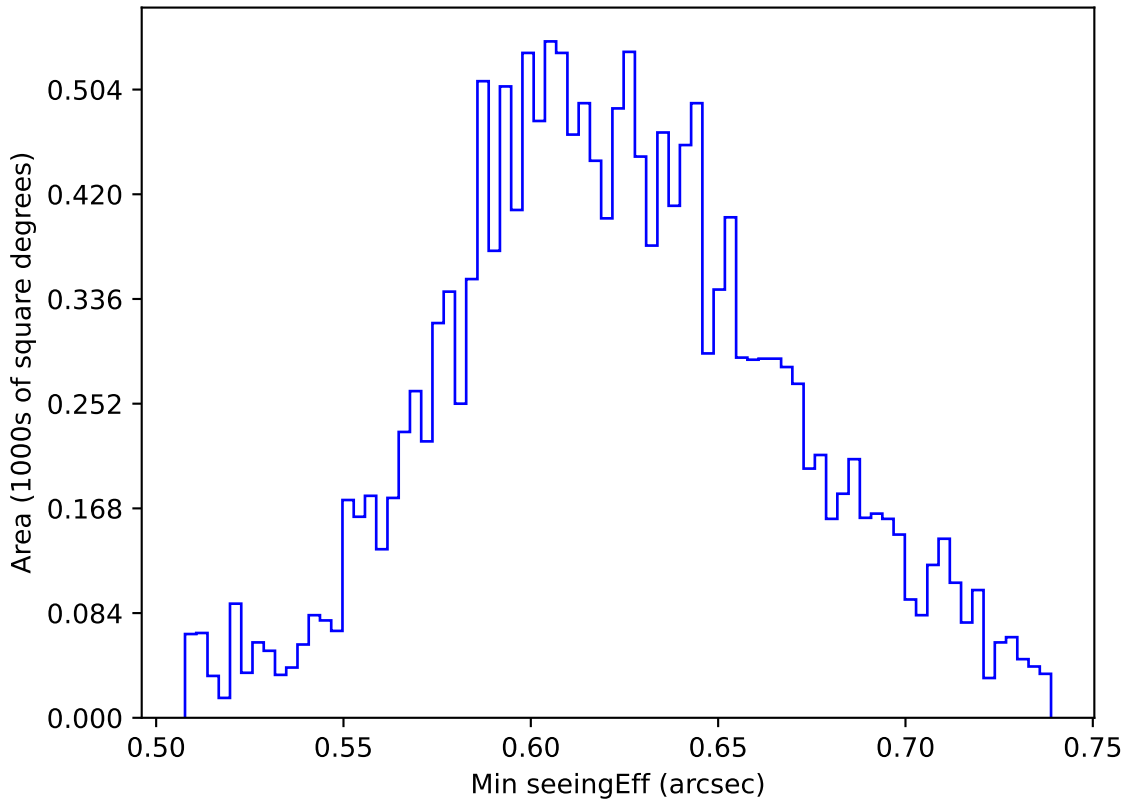
too_elab_heavy_r32_d2_ugrizy_v3.4_10yrs WFD y band: Min seeingEff
