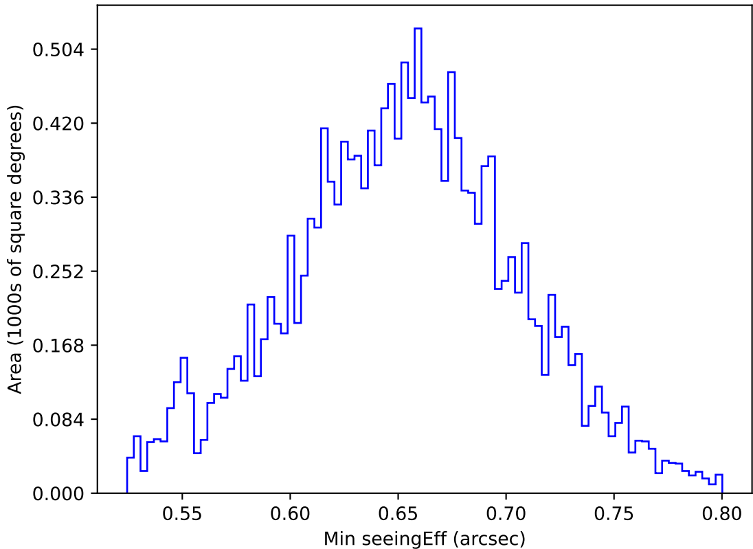
too_elab_heavy_r32_d2_ugrizy_v3.4_10yrs WFD g band: Min seeingEff
