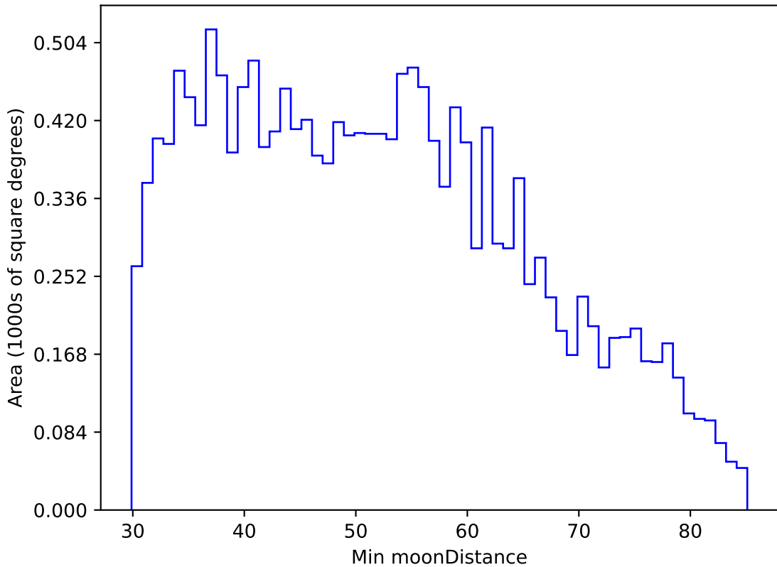
too_elab_heavy_r32_d2_ugrizy_v3.4_10yrs WFD u band: Min moonDistance
