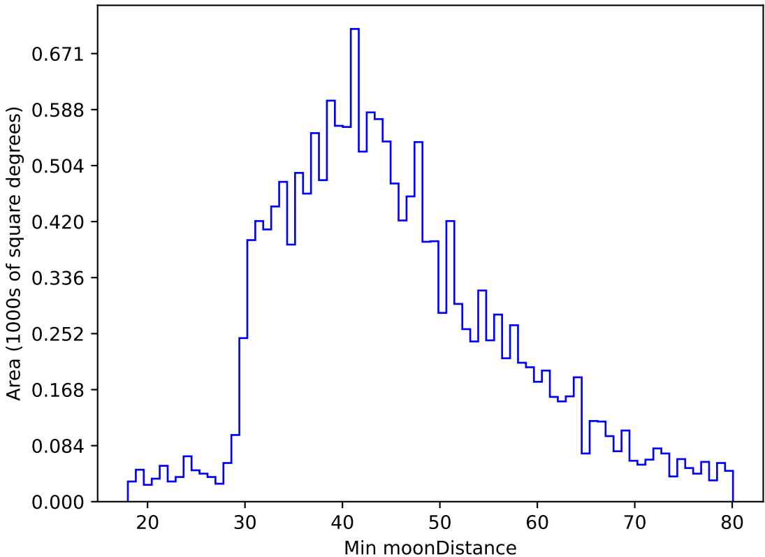
too_elab_heavy_r32_d2_ugrizy_v3.4_10yrs WFD g band: Min moonDistance
