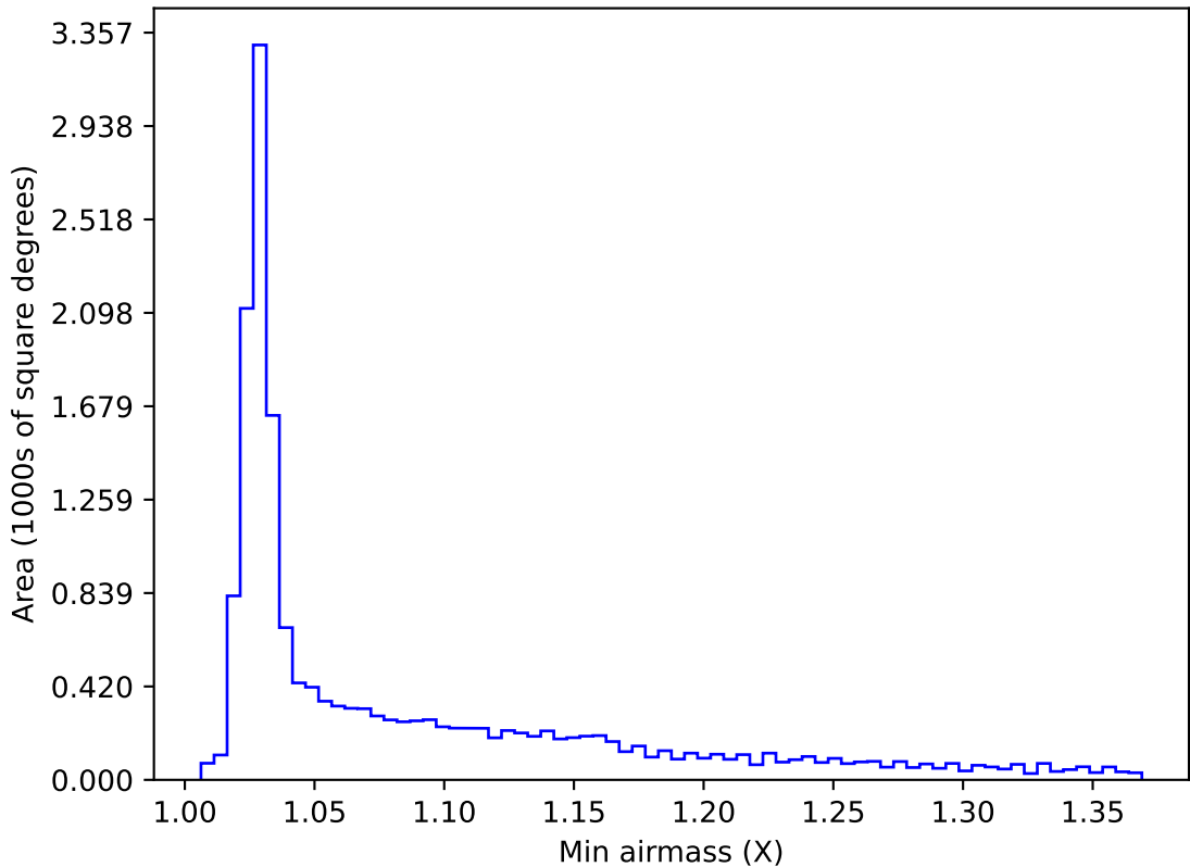
too_elab_heavy_r32_d2_ugrizy_v3.4_10yrs WFD i band: Min airmass
