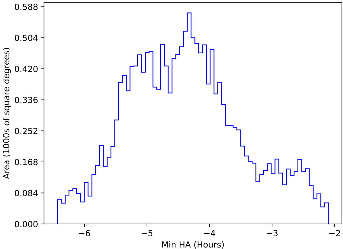
too_elab_heavy_r32_d2_ugrizy_v3.4_10yrs WFD z band: Min HA
