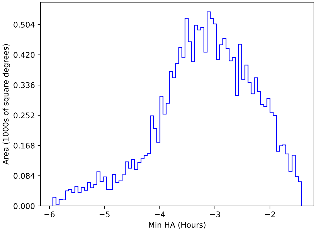
too_elab_heavy_r32_d2_ugrizy_v3.4_10yrs WFD u band: Min HA
