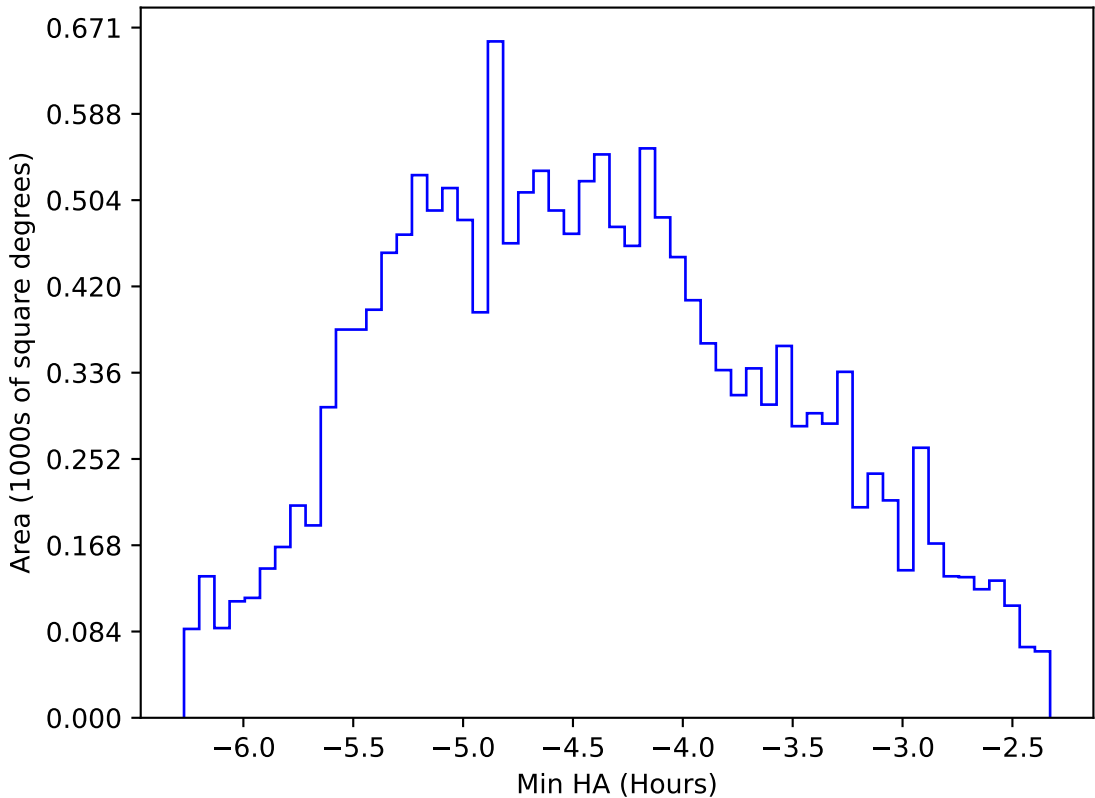
too_elab_heavy_r32_d2_ugrizy_v3.4_10yrs WFD r band: Min HA
