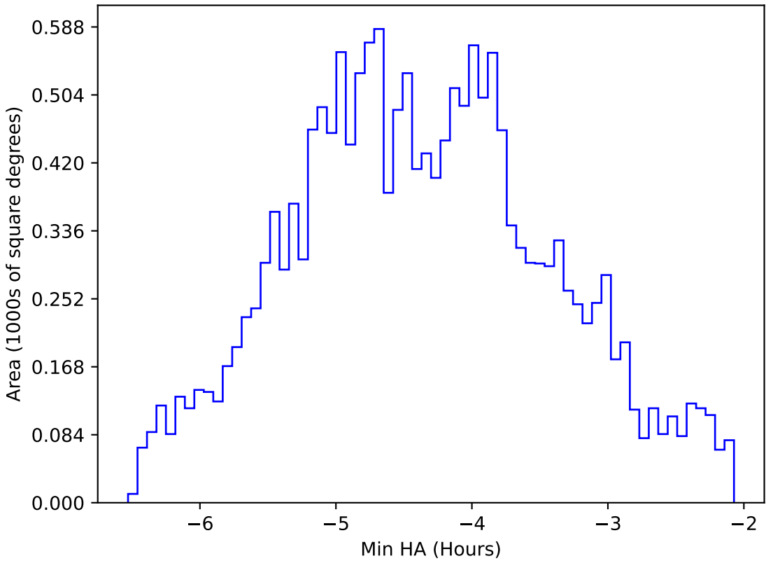
too_elab_heavy_r32_d2_ugrizy_v3.4_10yrs WFD i band: Min HA
