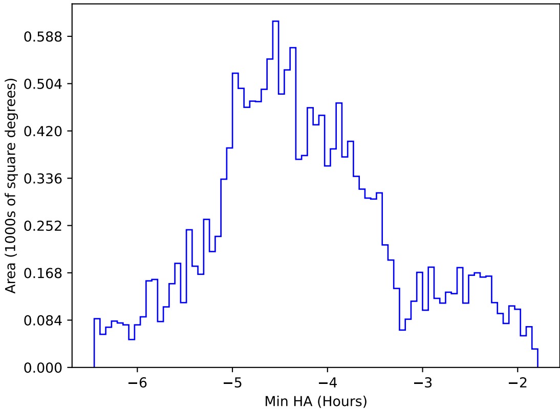
too_elab_heavy_r32_d2_ugrizy_v3.4_10yrs WFD g band: Min HA
