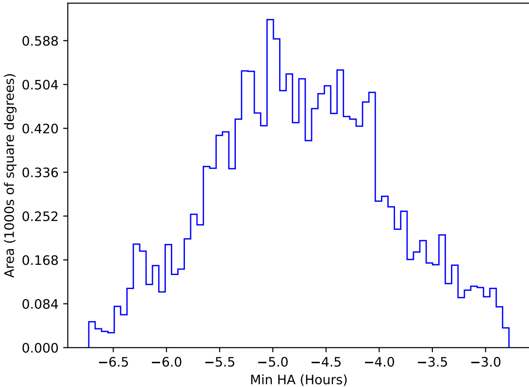
too_elab_heavy_r32_d2_ugrizy_v3.4_10yrs WFD all bands: Min HA
