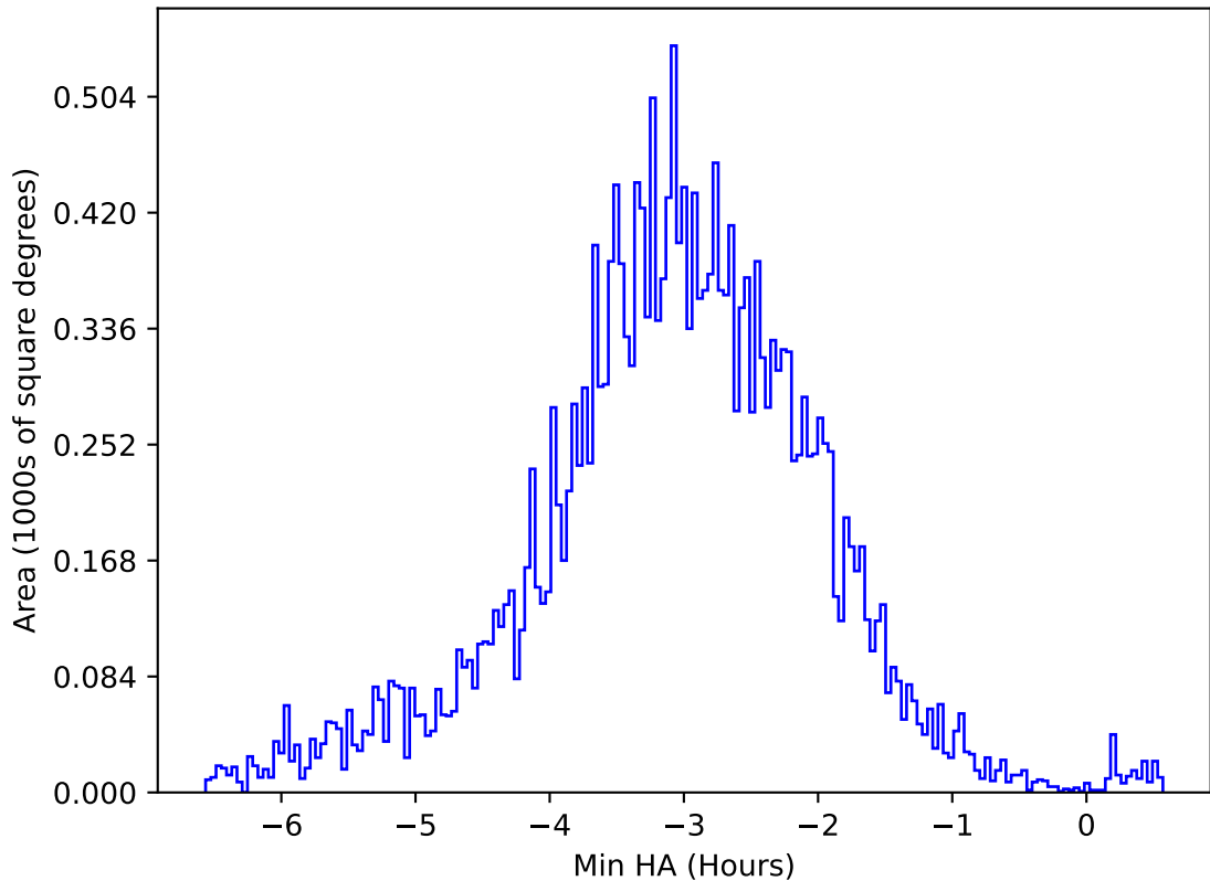
too_elab_heavy_r32_d2_ugrizy_v3.4_10yrs All sky u band: Min HA
