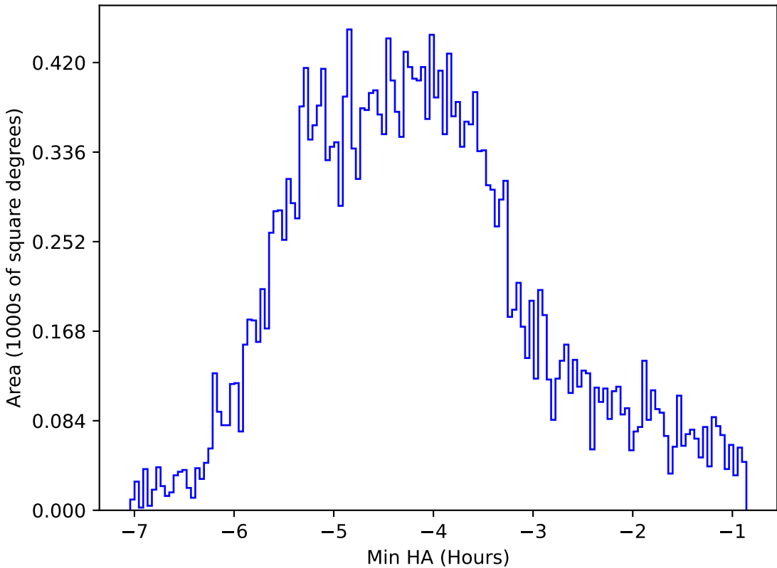
too_elab_heavy_r32_d2_ugrizy_v3.4_10yrs All sky r band: Min HA
