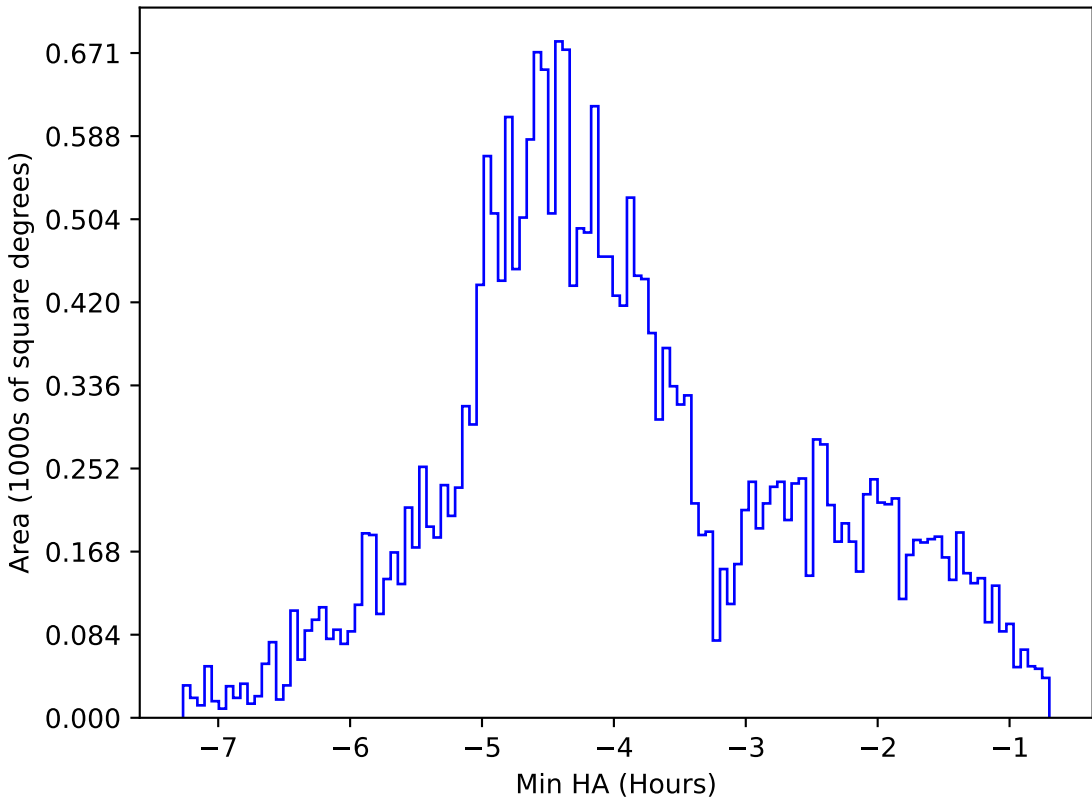
too_elab_heavy_r32_d2_ugrizy_v3.4_10yrs All sky g band: Min HA
