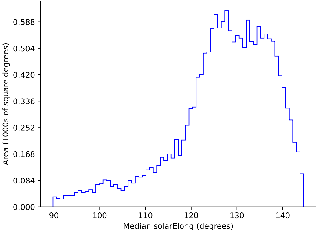
too_elab_heavy_r32_d2_ugrizy_v3.4_10yrs WFD z band: Median solarElong
