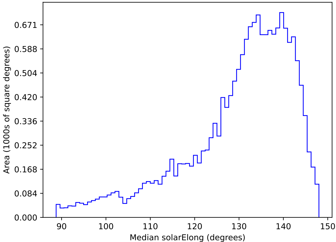
too_elab_heavy_r32_d2_ugrizy_v3.4_10yrs WFD y band: Median solarElong
