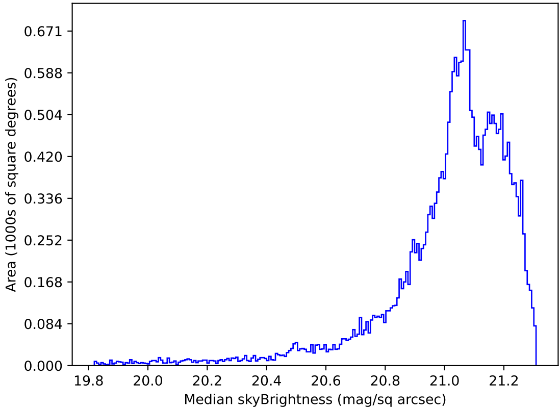
too_elab_heavy_r32_d2_ugrizy_v3.4_10yrs Yr 1 r band: Median skyBrightness
